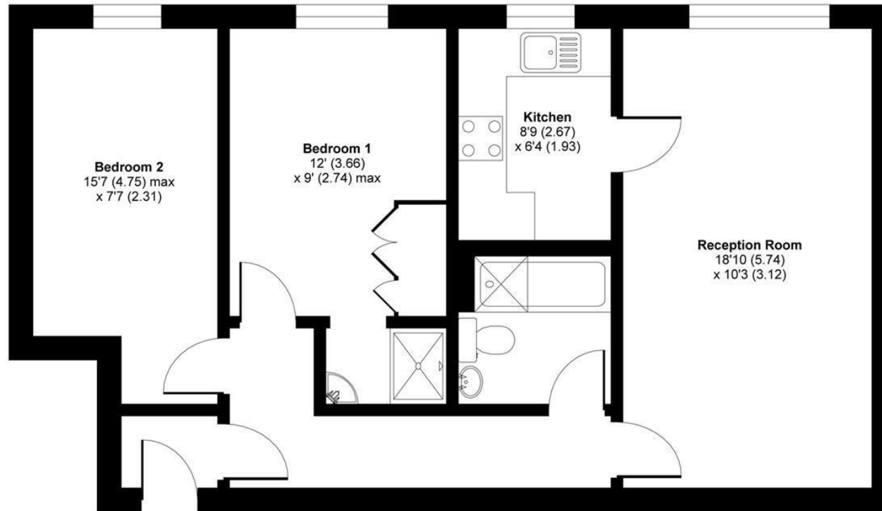
THIRD FLOOR
